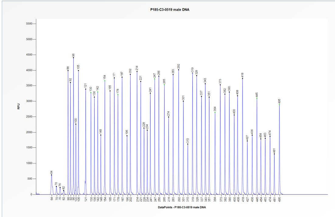
Figure 1. Capillary electrophoresis pattern from a sample of approximately 50 ng human male control DNA analysed with SALSA MLPA Probemix P185 Intersex (C3-0519).
