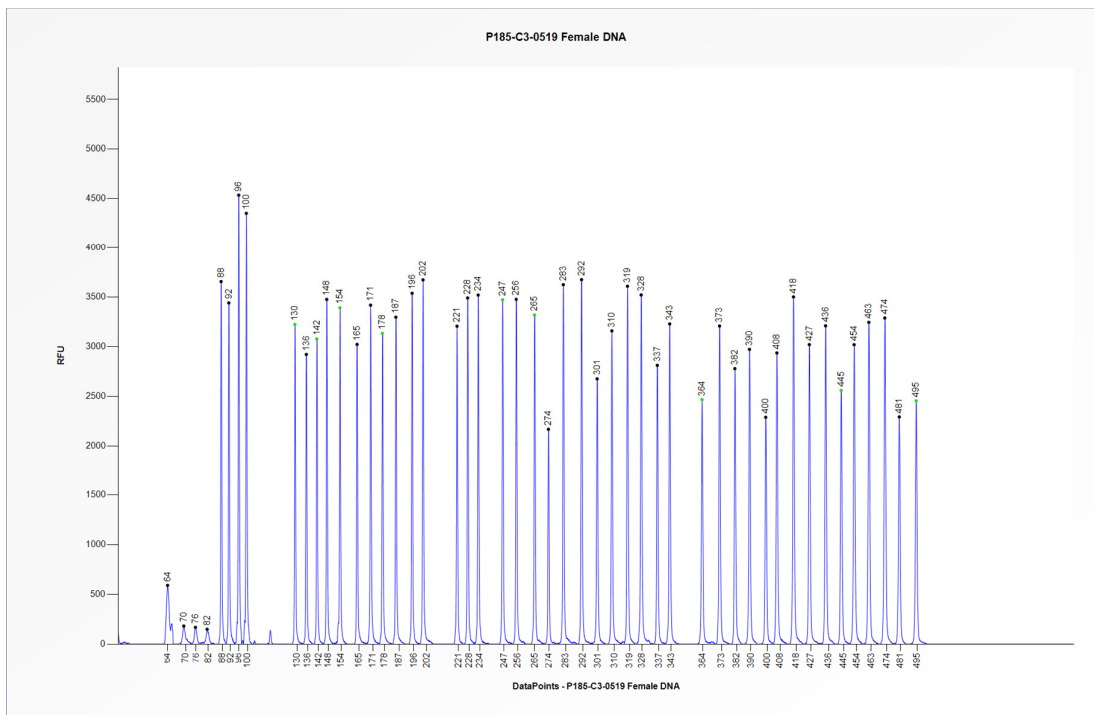
Figure 2. Capillary electrophoresis pattern from a sample of approximately 50 ng human female control DNA analysed with SALSA MLPA Probemix P185 Intersex (C3-0519).
