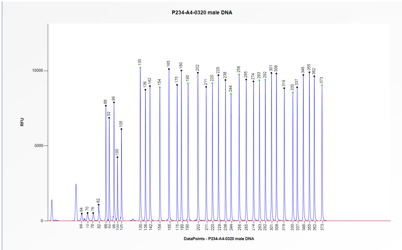
Figure 1. Capillary electrophoresis pattern from a sample of approximately 50 ng human male control DNA analysed with SALSA MLPA Probemix P234 GATA3 - GATA4 (A4-0320).
