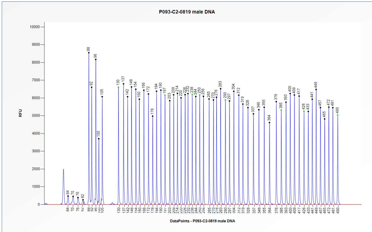
Figure 1. Capillary electrophoresis pattern from a sample of approximately 50 ng human male control DNA analysed with SALSA MLPA Probemix P093 HHT/HPAH (C2-0819).
