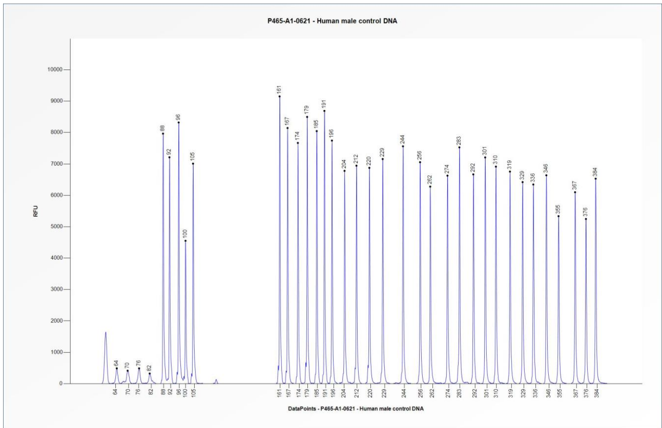
Figure 1. Capillary electrophoresis pattern from a sample of approximately 50 ng human male control DNA analysed with SALSA MLPA Probemix P465 ACADM (A1-0621).
