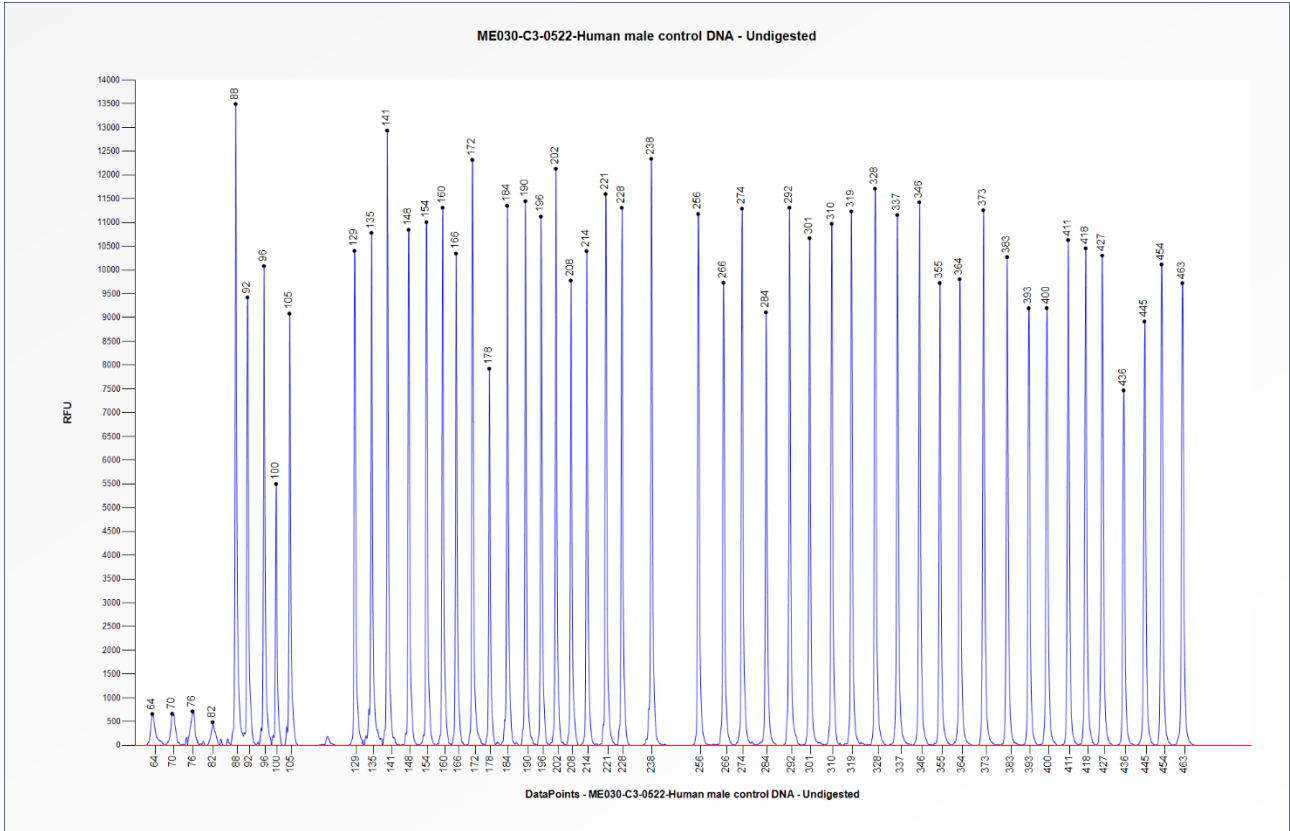
Figure 1. Capillary electrophoresis pattern from a sample of approximately 50 ng undigested human male control DNA analysed with SALSA MS-MLPA Probemix ME030 BWS/RSS (C3-0522) for the quantification of copy numbers.
