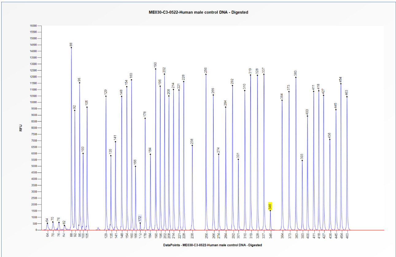
Figure 2. Capillary electrophoresis pattern from a sample of approximately 50 ng digested human male control DNA analysed with SALSA MS-MLPA Probemix ME030 BWS/RSS (C3-0522) to determine the methylation status.
