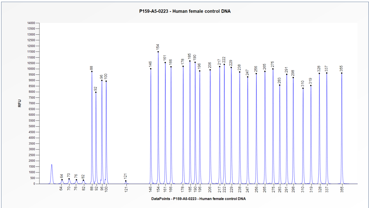
Figure 2 Capillary electrophoresis pattern from a sample of approximately 50 ng human female control DNA analysed with SALSA MLPA Probemix P159 GLA (A5-0223).
