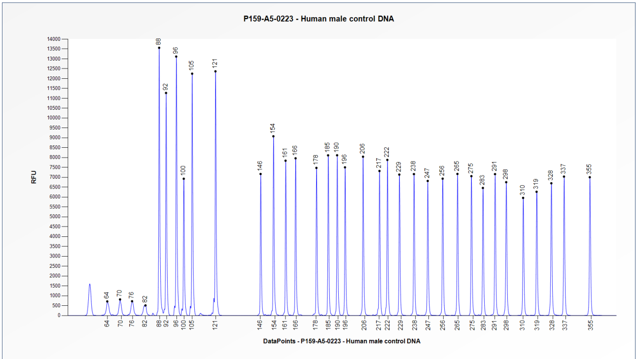
Figure 1. Capillary electrophoresis pattern from a sample of approximately 50 ng human male control DNA analysed with SALSA MLPA Probemix P159 GLA (A5-0223).
