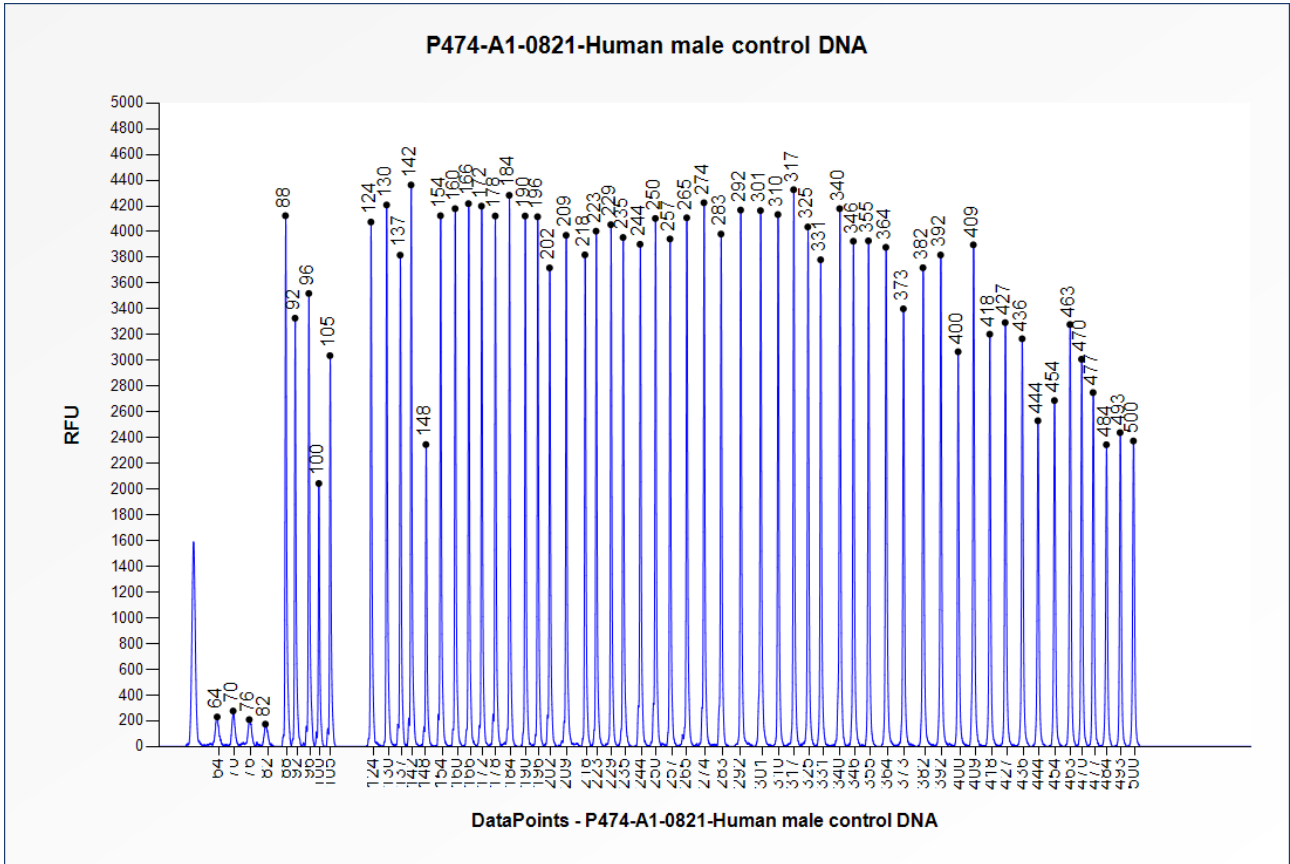
Figure 1. Capillary electrophoresis pattern from a sample of approximately 50 ng human male control DNA analysed with SALSA MLPA Probemix P474 CD274-PDCD1LG2-JAK2 (A1-0821).
