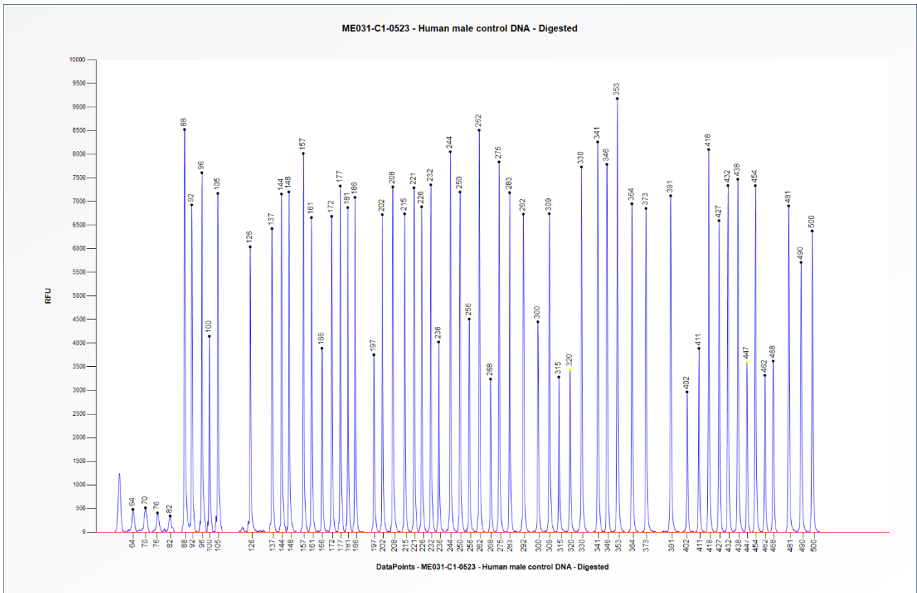
Figure 2. Capillary electrophoresis pattern from a sample of approximately 50 ng digested human male control DNA analysed with SALSA MS-MLPA Probemix ME031 GNAS (C1-0523) to determine the methylation status.
