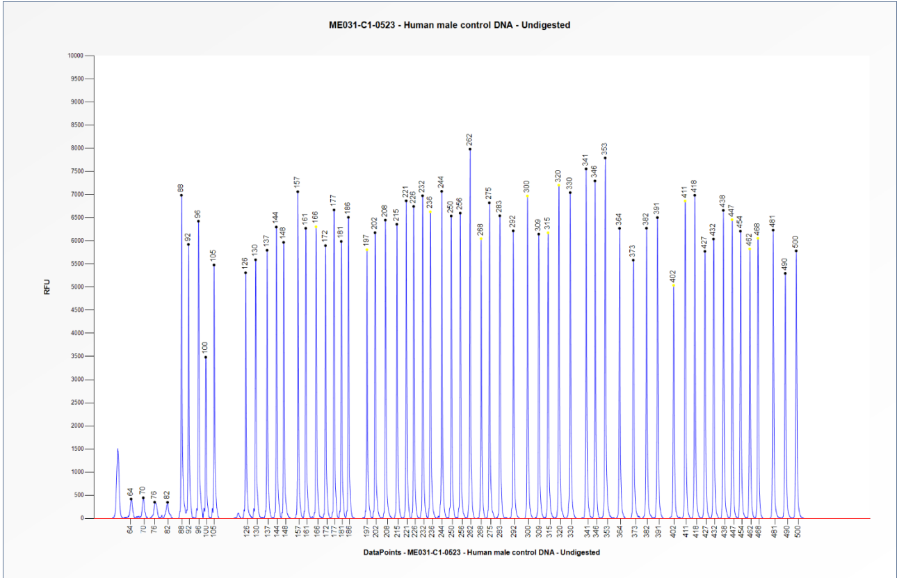
Figure 1. Capillary electrophoresis pattern from a sample of approximately 50 ng undigested human male control DNA analysed with SALSA MS-MLPA Probemix ME031 GNAS (C1-0523) for the quantification of copy numbers.
